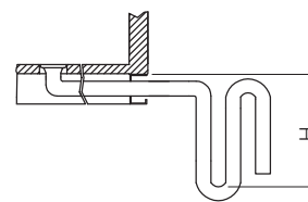
Positive pressure siphon - bottom connection:
