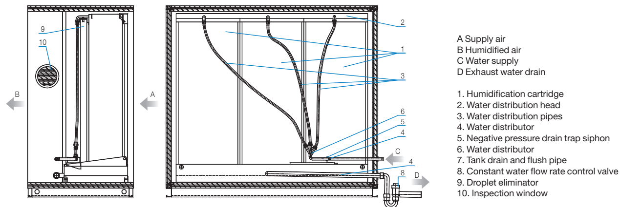
Honeycomb humidifier with direct water
