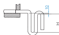
Positive pressure siphon - side connection:
